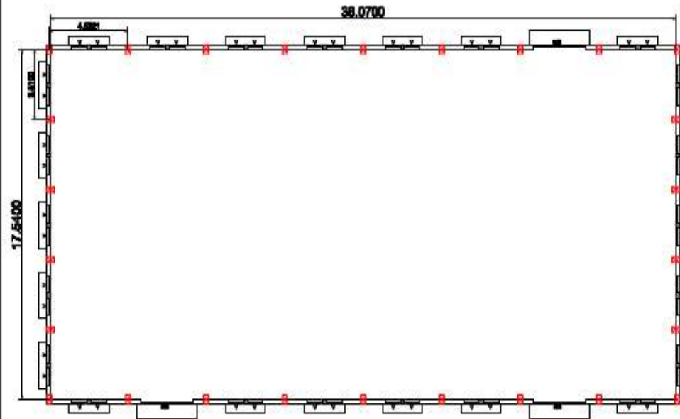
GODOWN PLAN scale 1:100 SIZE 36.07 M X 17.54 M X 6.00 M
