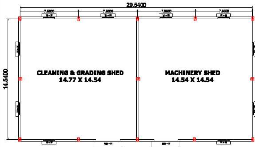
CLEANING & MACHINERY SHED scale 1:100 SIZE 29.54M X 14.54 M X 12.05 M
